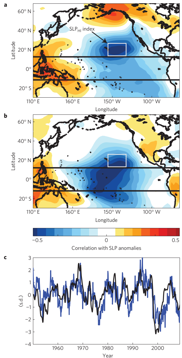
Figure 2 | The atmospheric forcing of the NPGO. a. Correlation of the NPGO index with monthly NCEP SLP anomalies. The SLP anomalies averaged over the white rectangle east of Hawaii are used to derive an index of the atmospheric forcing of the NPGO, referred to as the SLP HI index. b. Correlation map of the CPW index with NCEP SLP anomalies. c. The NPGO index (blue) is reconstructed (black) using an AR1 model forced by the SLP HI index. The units are in standard deviations (s.d.). The significance of correlation ( R = 0.65 ; >99%) of the raw monthly values is estimated using a Monte Carlo test for time series with a corresponding red spectra (see the Methods section).
