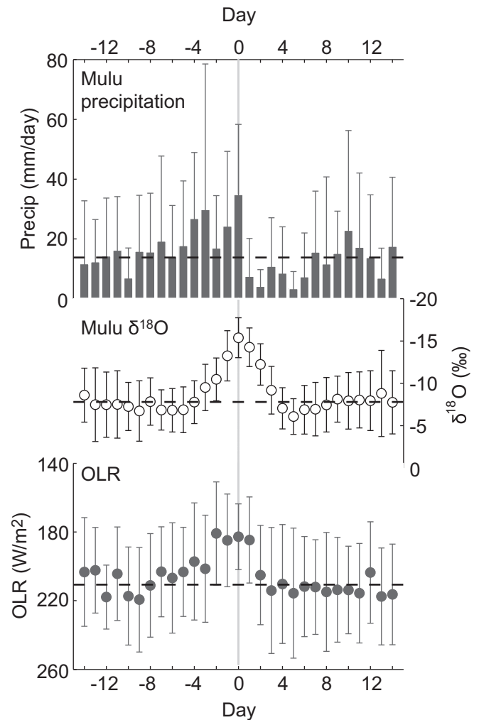
Fig. 6. Composites of (top) daily Mulu precipitation amount, (middle) daily Mulu rainfall \delta^{18}\text{O} , and (bottom) daily OLR at 5^\circ\text{N} , 115^\circ\text{E} during the eighteen intraseasonal rainfall \delta^{18}\text{O} depletion events centered about Day ‘0’, which represents the minimum rainfall \delta^{18}\text{O} value of the depletion events. Error bars reflect the 1\sigma spread for each daily average. Dashed horizontal lines represent the long-term daily average value of each parameter over the 5-yr study period ( 13.8 \pm 23.2 mm/day [ 1\sigma ] for local Mulu precipitation, -7.8 \pm 3.6\text{‰} [ 1\sigma ] for Mulu rainfall \delta^{18}\text{O} , and 210.7 \pm 30.4 \text{Wm}^{-2} [ 1\sigma ] for OLR). Note that axes for \delta^{18}\text{O} and OLR are inverted.
