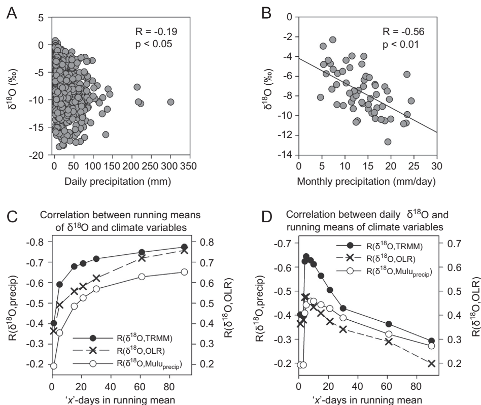
Fig. 4. (A) Relationship between daily Mulu rainfall \delta^{18}\text{O} and daily Mulu precipitation amount. (B) Relationship between monthly-averaged Mulu rainfall \delta^{18}\text{O} and monthly-averaged local Mulu precipitation amount. Solid black line represents linear best fit. (C) Correlation between 'x'-day running mean Mulu rainfall \delta^{18}\text{O} and 'x'-day running means of Mulu precipitation amount (open circles, solid line), satellite-derived TRMM 3B42 precipitation amount (black circles, solid line), and NOAA interpolated OLR (black crosses, dashed line). (D) Correlation between daily Mulu rainfall \delta^{18}\text{O} and 'x'-day minus-projected running means of local Mulu precipitation amount (open circles, solid line), TRMM 3B42 precipitation amount (black circles, solid line), and OLR (black crosses, dashed line), after Risi et al. (2008a). TRMM and OLR in both (C) and (D) are spatial averages integrated over a 2.5^\circ \times 2.5^\circ gridbox centered about 5^\circ\text{N} , 115^\circ\text{E} .
