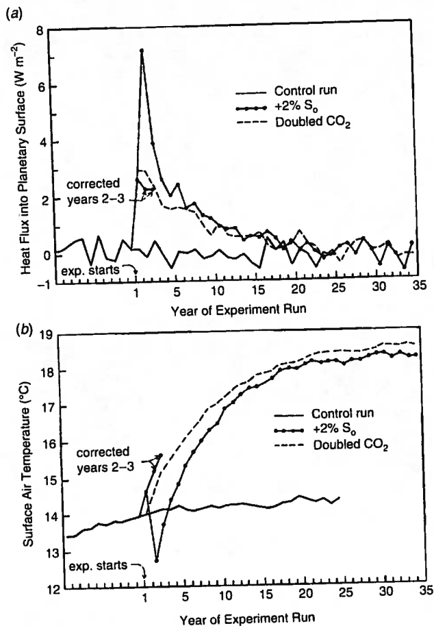
Fig. 3. Global net heat flux into planetary surface (a) and global surface air temperature (b). On April 1 of year 2 in the S 0 experiment the computer was hit by a cosmic ray or some other disturbance which caused improper numbers to be stored in the ground temperature array. This affected the temporal development of that run, but should not influence its equilibrium results. In order to determine the maximum heat flux into the ocean, the S 0 experiment was rerun for years 2 and 3 from March 31 year 2 thus eliminating the computer error for that period.
