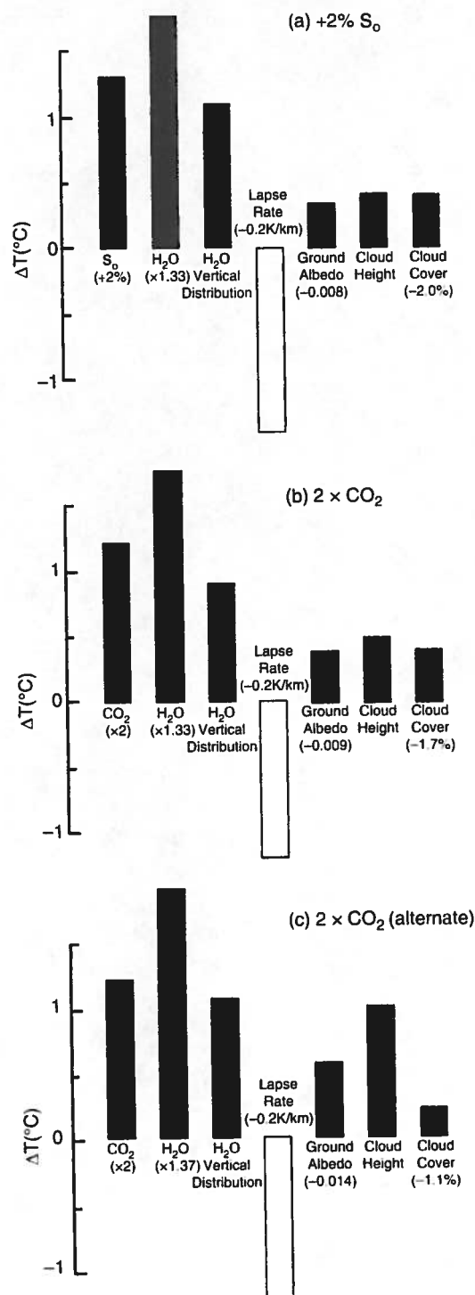
Fig. 6. Contributions to the global mean temperature rise in the S_0 and \text{CO}_2 experiments as estimated by inserting changes obtained in the 3-D experiments into 1-D radiative convective model. (a) +2 percent S_0 experiment, (b) doubled \text{CO}_2 experiment, and (c) doubled \text{CO}_2 experiment for alternate control run with greater sea ice.
