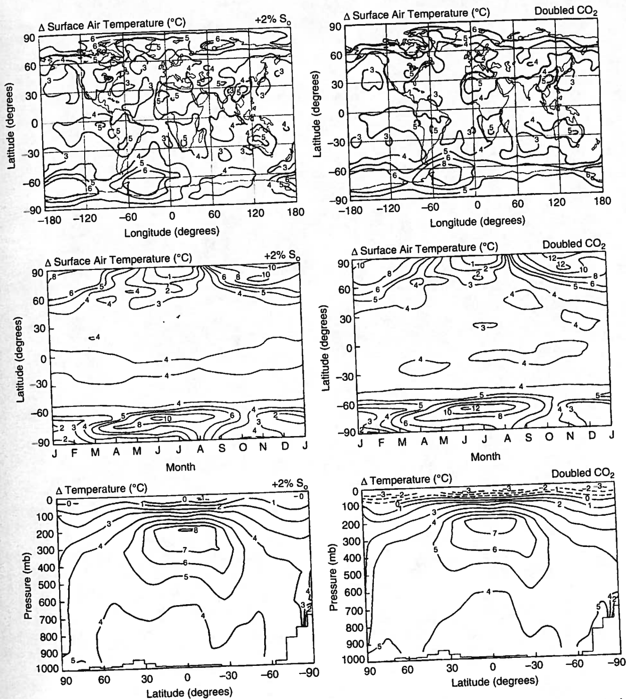
Fig. 4. Air temperature change in the climate model for a two percent increase of solar irradiance (left) and for doubled atmospheric CO_2 (right). The upper graphs show the geographical distribution of annual mean surface air warming, the middle graphs show the seasonal variation of the surface air warming averaged over longitude, and the lower graphs show the altitude distribution of the temperature change averaged over season and longitude.
