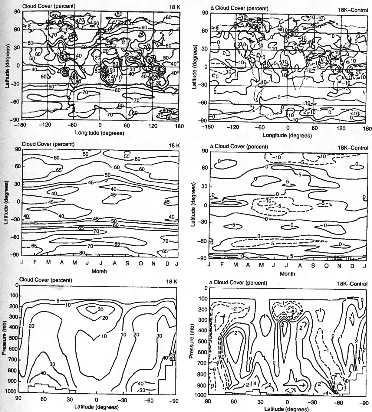
Fig. 11. Cloud cover for the 18K simulation and differences with the control run. The control run is described in detail in paper 1.
