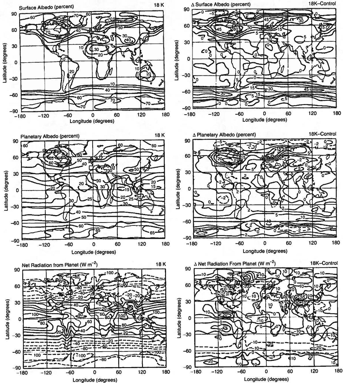
Fig. 10. Radiation quantities for the 18K simulation and differences with the control run. The control run is described in detail in paper 1.
