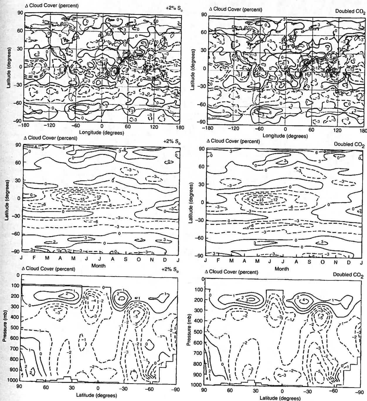
Fig. 8. Cloud changes in the climate model for two percent increase of S_0 (left) and doubled CO_2 (right). The upper graphs show the geographical distribution of annual mean cloud cover change, the middle graphs show the seasonal variation of cloud cover change averaged over longitude, and the lower graphs show the altitude distribution of the cloud cover change averaged over season and longitude.
