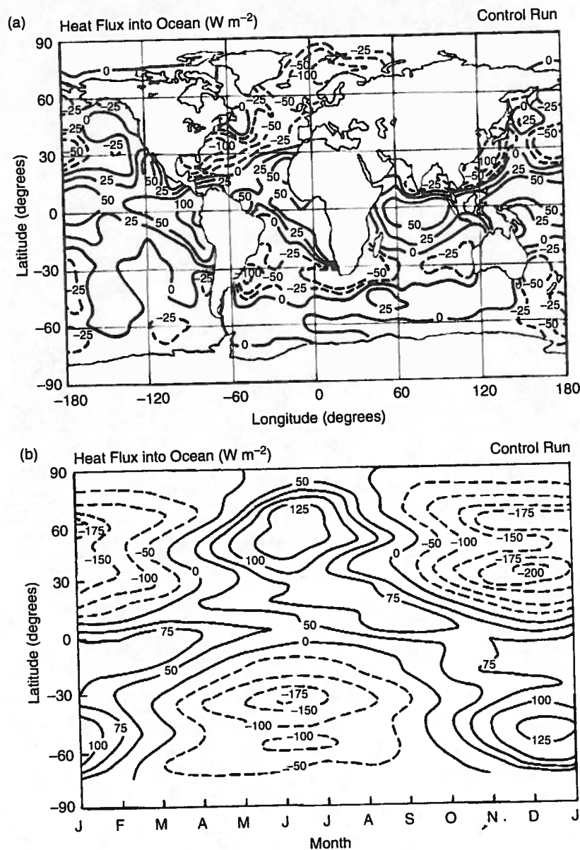
Fig. 1. Specified heat flux into the ocean surface in the 3-D climate model experiments, obtained from the model II run of paper 1 which had specified climatological seasonally-varying ocean surface temperature and ocean ice cover. (a) is the geographical distribution of the annual-mean flux. (b) is the latitude/season distribution of the zonal-mean flux.
