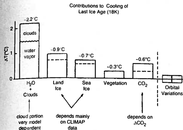
Fig. 13. Contributions to the global mean temperature difference between the Wisconsin ice age and today's climate as evaluated with a 3-D climate model and assumed boundary conditions. The cloud and water vapor portions were not separated, but based on other 3-D experiments the cloud part is estimated as 30–40 percent of their sum. The dashed line for land ice refers to the 'minimal extent' model of CLIMAP, and the dashed line for sea ice refers to the reduced sea ice cover in the Southern Hemisphere in experiments 11 and 11*. \Delta T_{\text{CO}_2} = 0.6^\circ\text{C} refers to a \text{CO}_2 change from 200 ppm (at 18K) to 300 ppm (at say 1900); this is reduced to 0.3^\circ\text{C} if the \text{CO}_2 amount was 225 ppm at 18K and 275 ppm at 1900.
