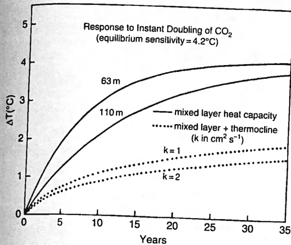
Fig. 16. Transient response to step function doubling of atmospheric CO 2 from 315 ppm to 630 ppm, computed from (24) with three representations of the ocean. The 63 m mixed layer corresponds to the mean mixed layer depth in the 3-D experiments; 110 m is the global-mean annual maximum mixed layer depth obtained from global ocean data. The curves including diffusion beneath the mixed layer are not exponentials (Appendix A).
