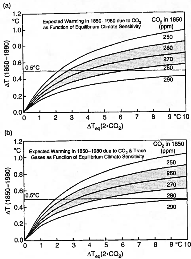
Fig. 17. Computed global warming between 1850 and 1980 as a function of the equilibrium climate sensitivity for doubled \text{CO}_2 (315 ppm \rightarrow 630 ppm), \Delta T_{\text{eq}} (2 \cdot \text{CO}_2) . Results are shown for five values of the assumed abundance of \text{CO}_2 in 1850; the shaded area covers the range 270 \pm 10 ppm recommended by WMO (1983). (a) includes only \text{CO}_2 growth, while (b) also includes the trace gas growths of Table 4. In all cases \text{CO}_2 increases linearly from the 1850 abundance to 315 ppm in 1958 and then according to measurements of Keeling et al. (1982).
