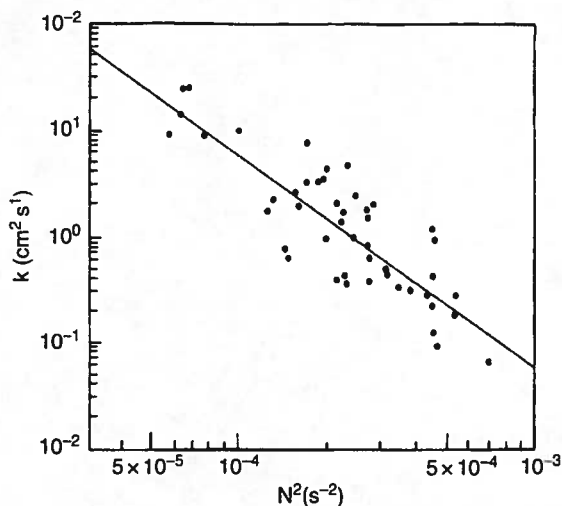
Fig. 14. Relationship between the effective diffusion coefficient ( k ) and the stability ( N^2 , where N is the Brunt-Vaisala frequency) at the base of the winter mixed layer for the GEOSECS tritium stations north of 20^\circ S . The regression line fit (Eq. 25) has correlation coefficient 0.85 with the points for individual stations.
