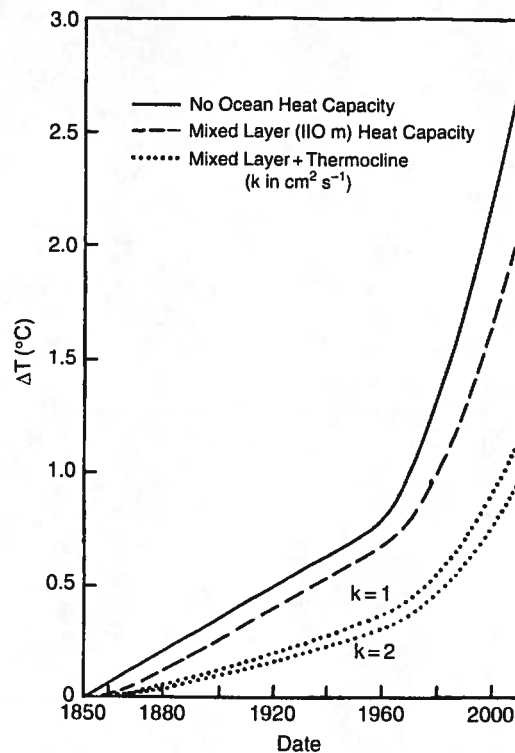
Fig. 18. Global mean warming computed for the \text{CO}_2 and trace gas scenarios in Table 4.
