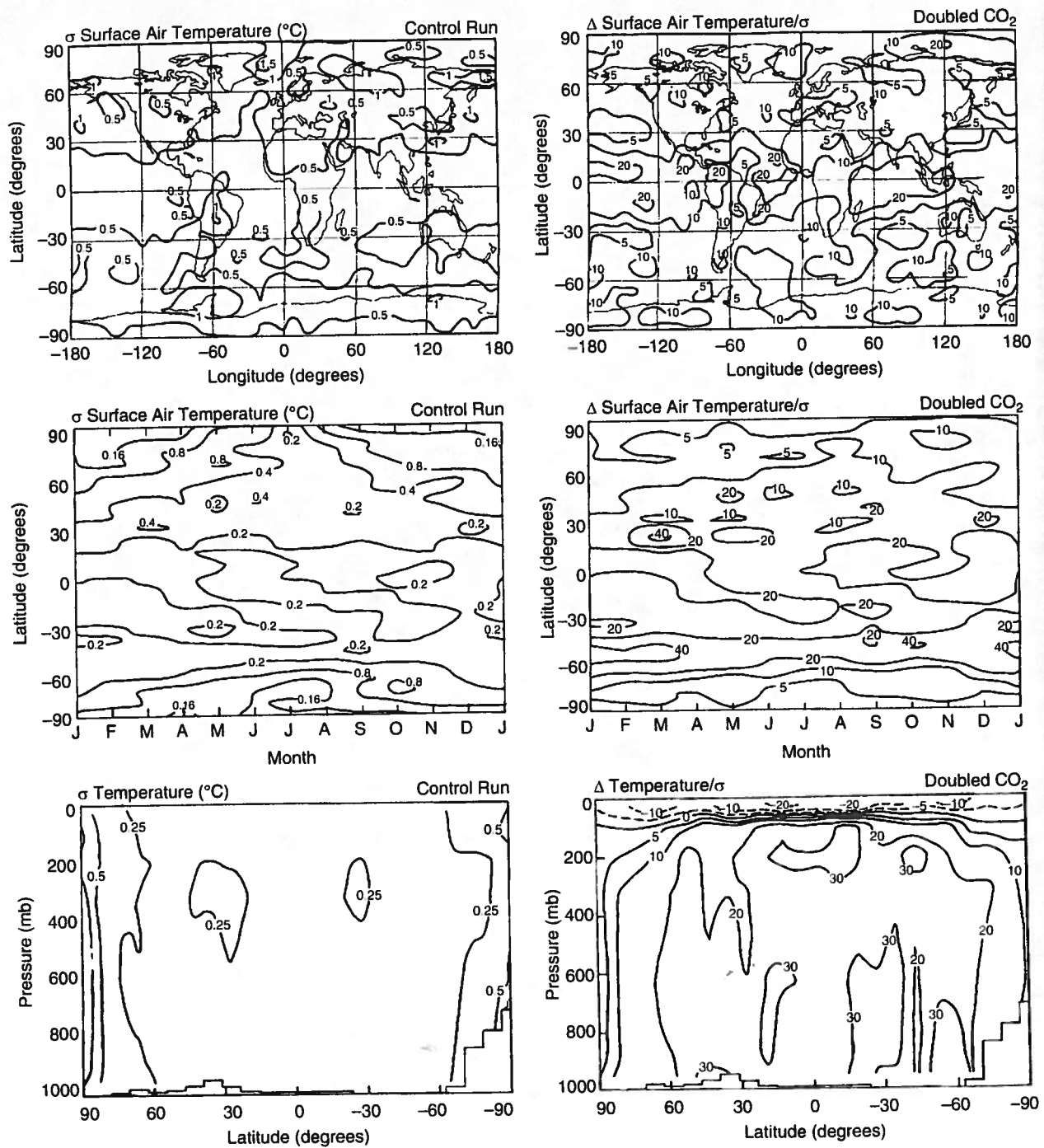
Fig. 5. Left side: standard deviation of temperature for the last 10 years in the control run. Right side: ratio of temperature change for years 26–35 of the doubled CO 2 experiment to the standard deviation of temperature in the control run.
