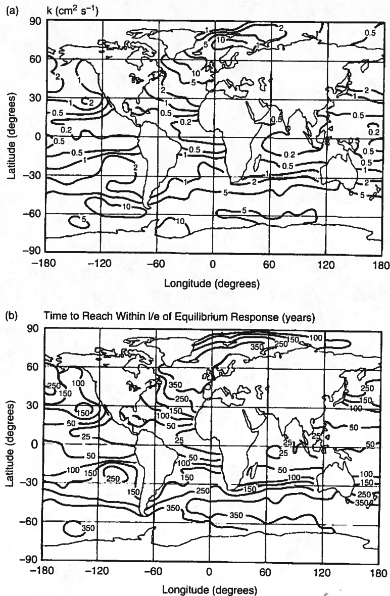
Fig. 15. (a) Geographic distribution of effective thermocline diffusion coefficient, k ( \text{cm}^2 \text{s}^{-1} ). k is derived from Eq. 25 and the global distribution of N^2 , the latter obtained from the ocean data of Levitus (1982). (b) Geographic distribution of the 63 percent response time for surface temperature response to doubled \text{CO}_2 in the atmosphere. Only geographic variability of k and mixed layer depth are accounted for. \Delta T_{\text{eq}} (2^* \text{CO}_2) is taken as 4.2^\circ\text{C} everywhere. The flux into the ocean is from Eq. (24).
