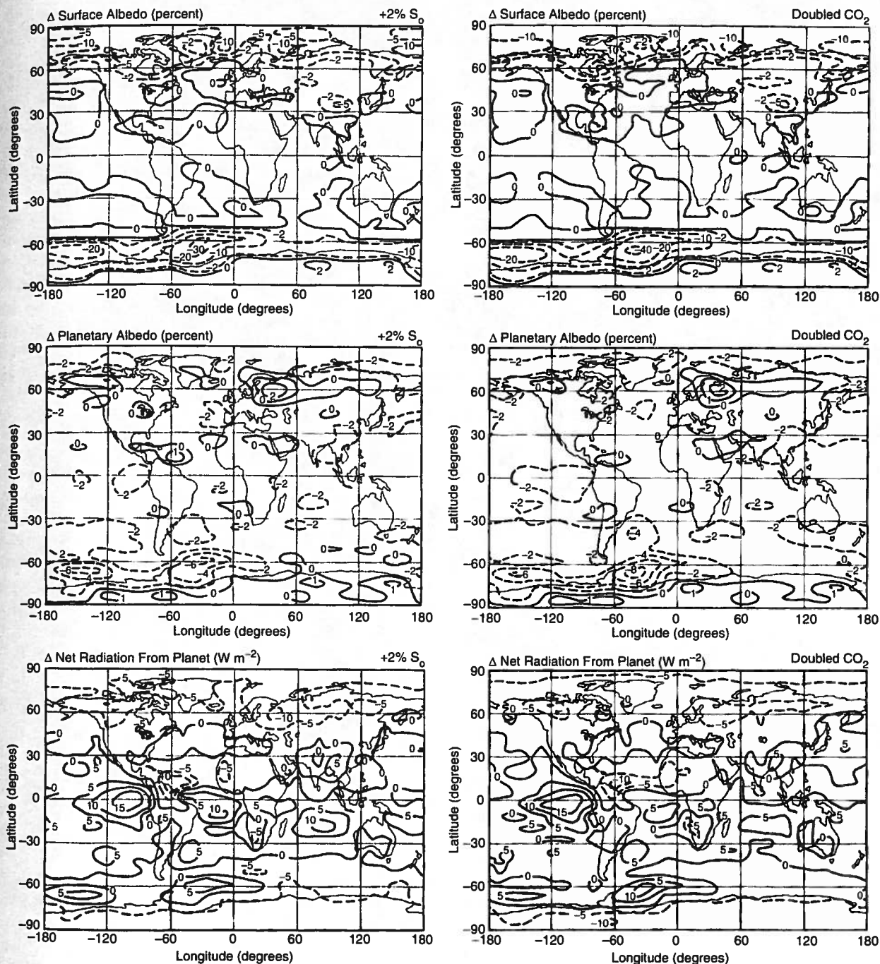
Fig. 7. Annual mean radiation changes in the climate model for two percent increase of S_0 (left) and doubled CO_2 (right). In Figs. 7, 8, 10 and 11 "percent" change refers to the full range of the quantity, e.g., a change from 60 percent albedo to 50 percent albedo is defined to be a 10 percent change.
